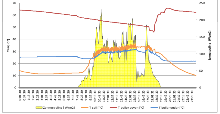
Datalogging Viessmann Vitosoll 300T - 30/09/10
