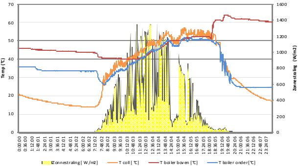
Datalogging Viessmann Vitosoll 300T - 24/08/10
