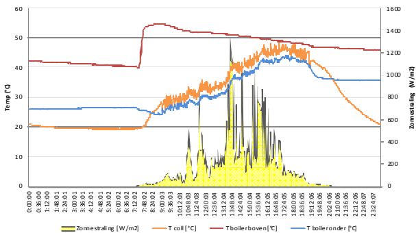
Datalogging Viessmann Vitosoll 300T - 23/08/10
