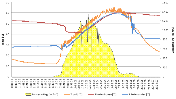
Datalogging Viessmann Vitosoll 300T - 20/08/10
