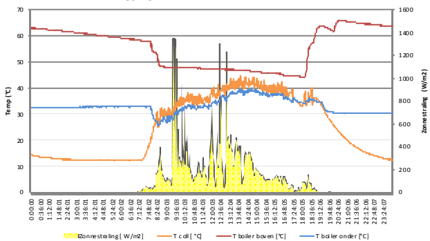
Datalogging Viessmann Vitosoll 300T - 29/08/10
